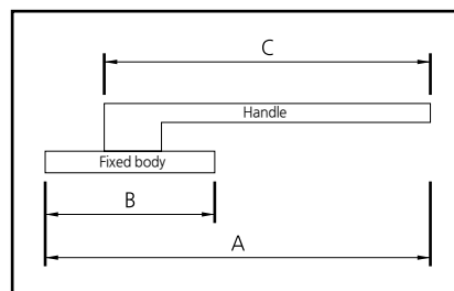
A1603 Grip handle (new type)
